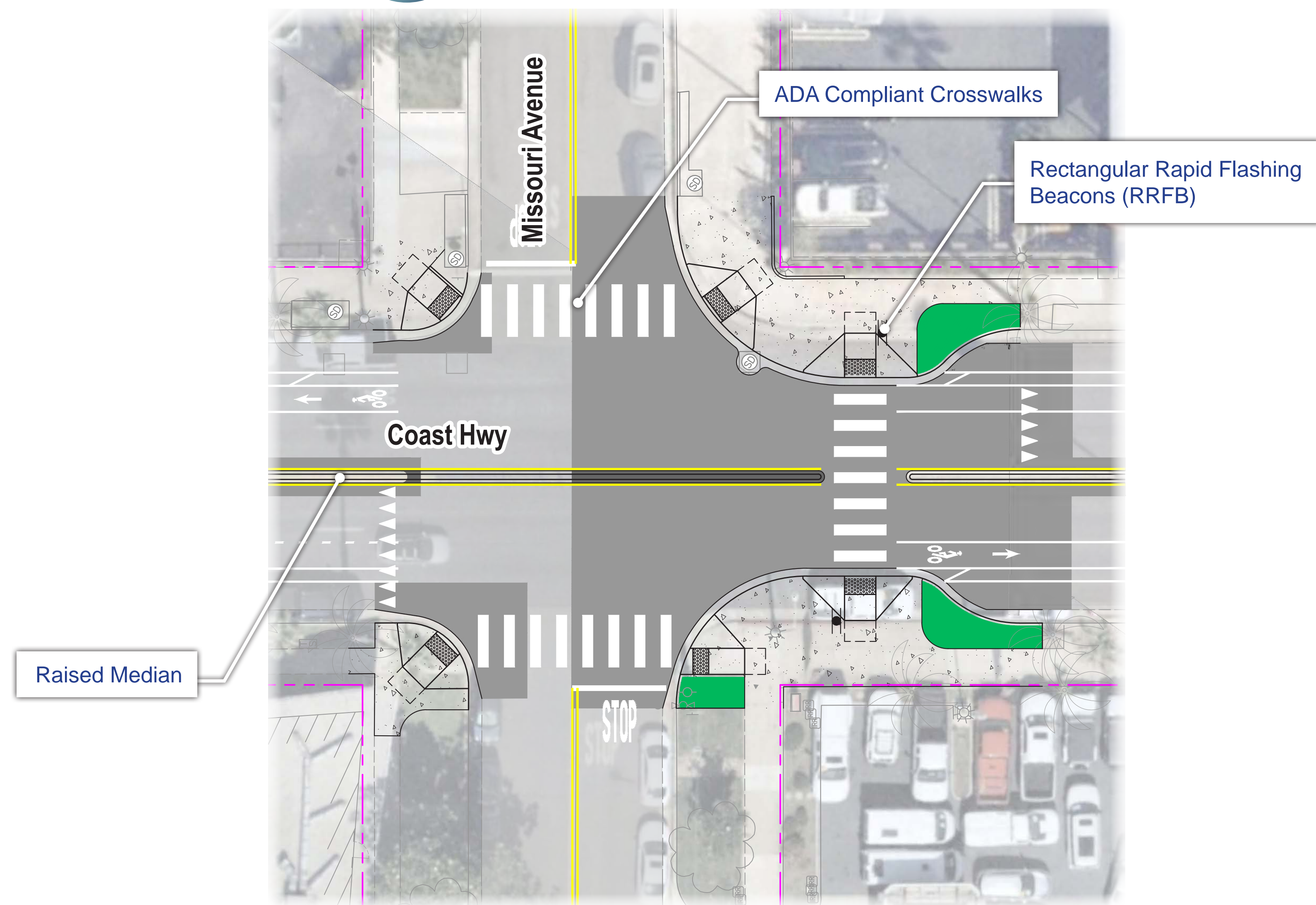
E MISSOURI AVE - BULB-OUTS
