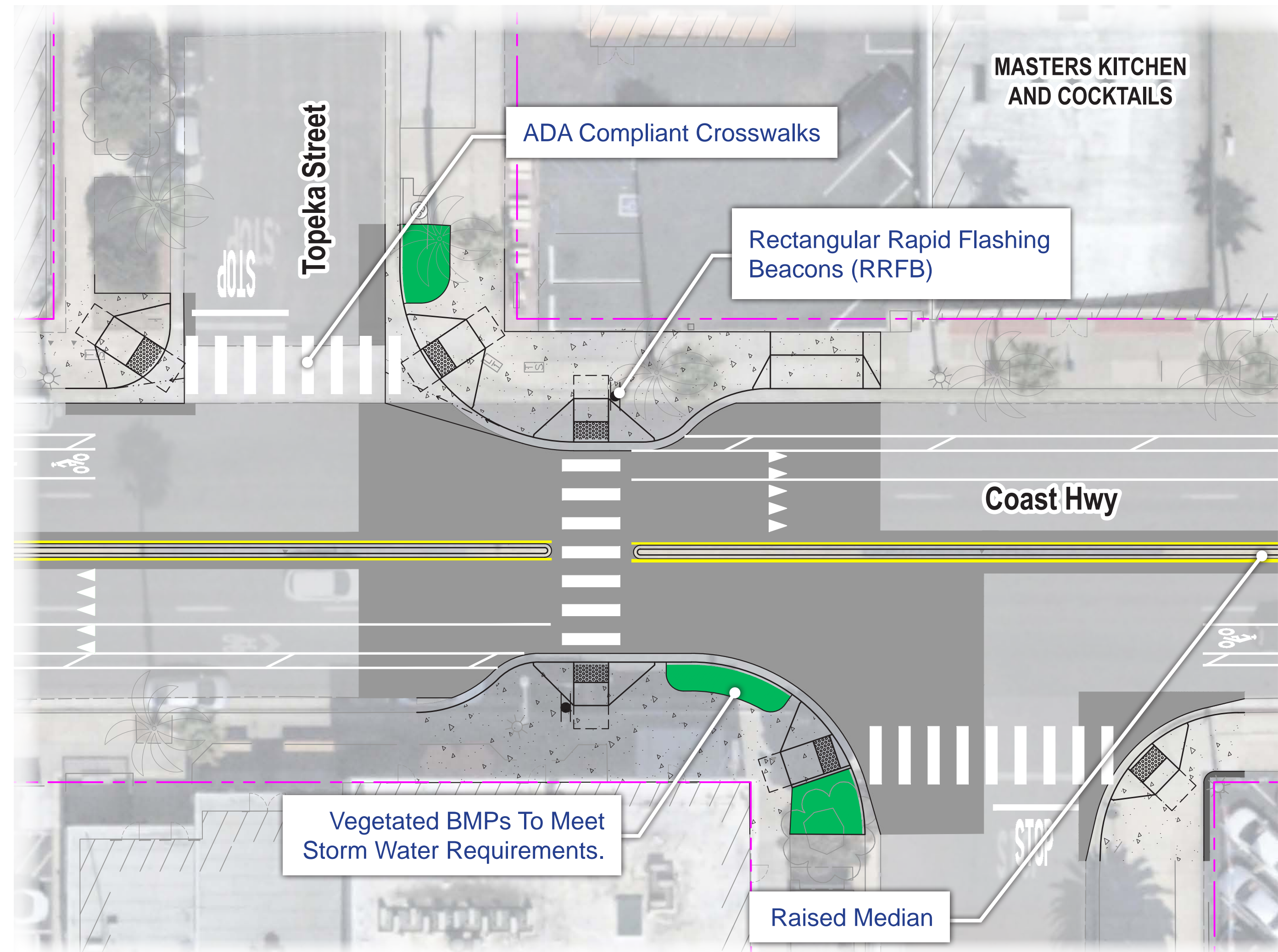
C TOPEKA STREET - BULB-OUTS
