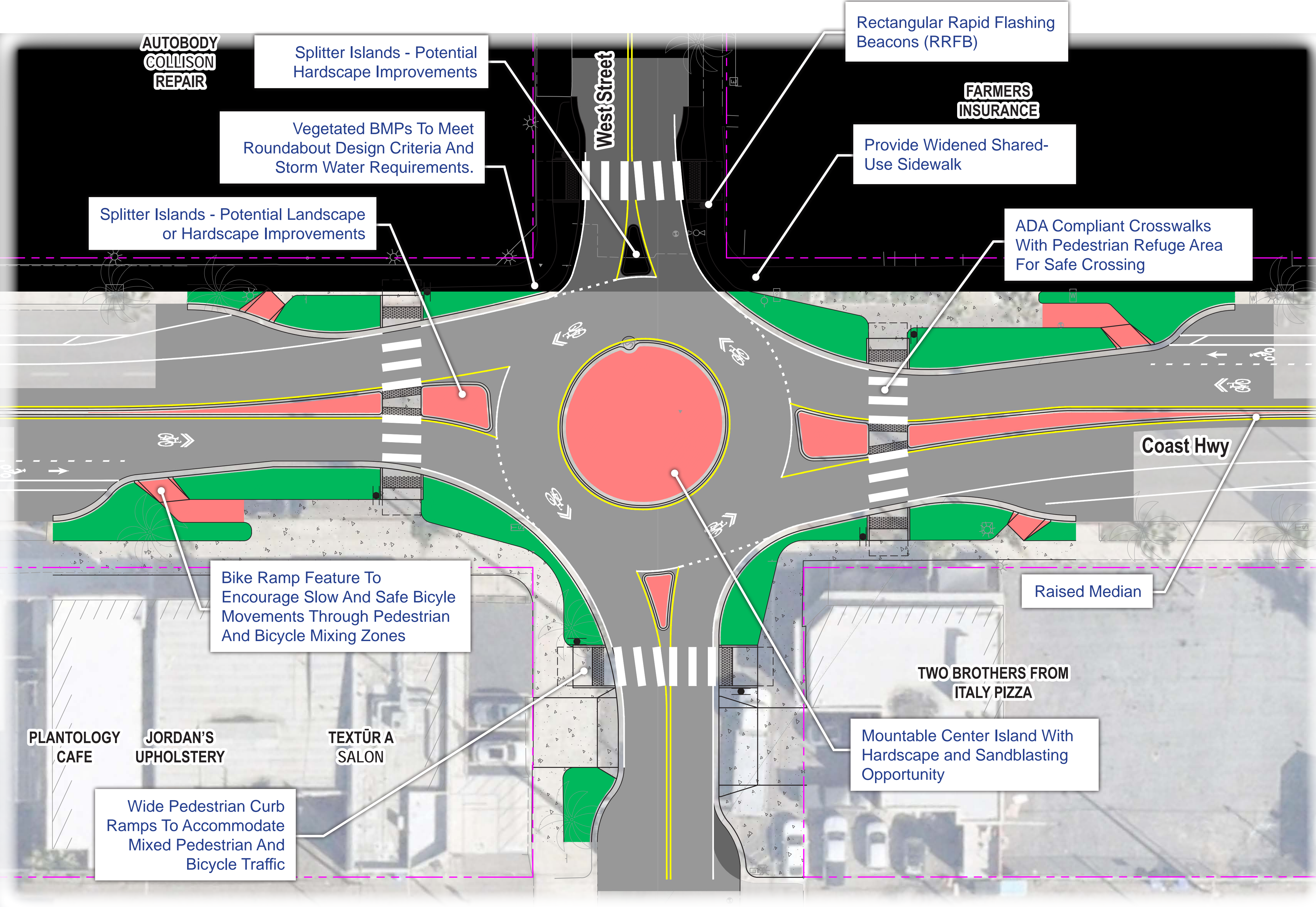
I WEST ST - ROUNDABOUT
