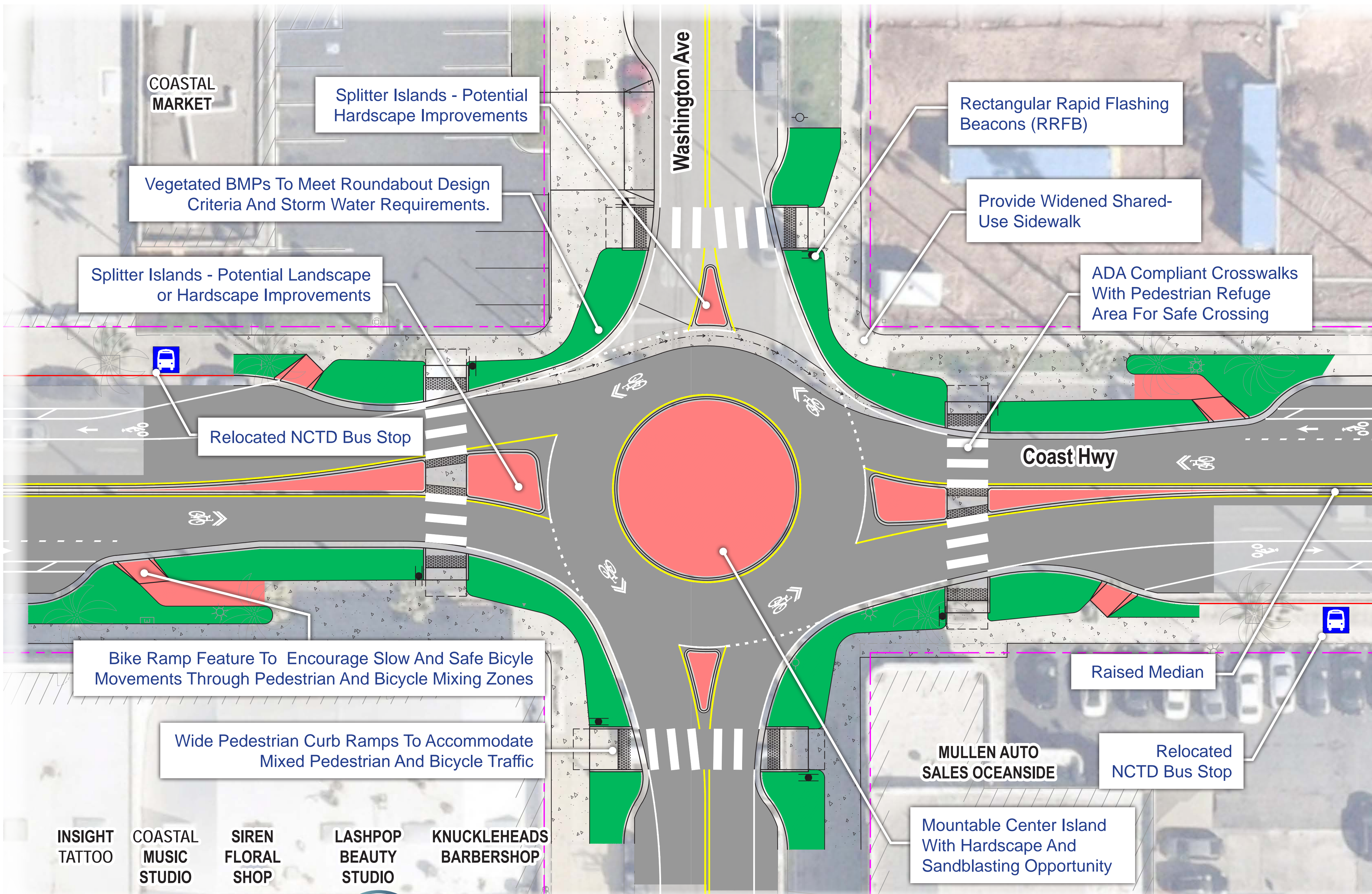
F WASHINGTON AVE - ROUNDABOUT
