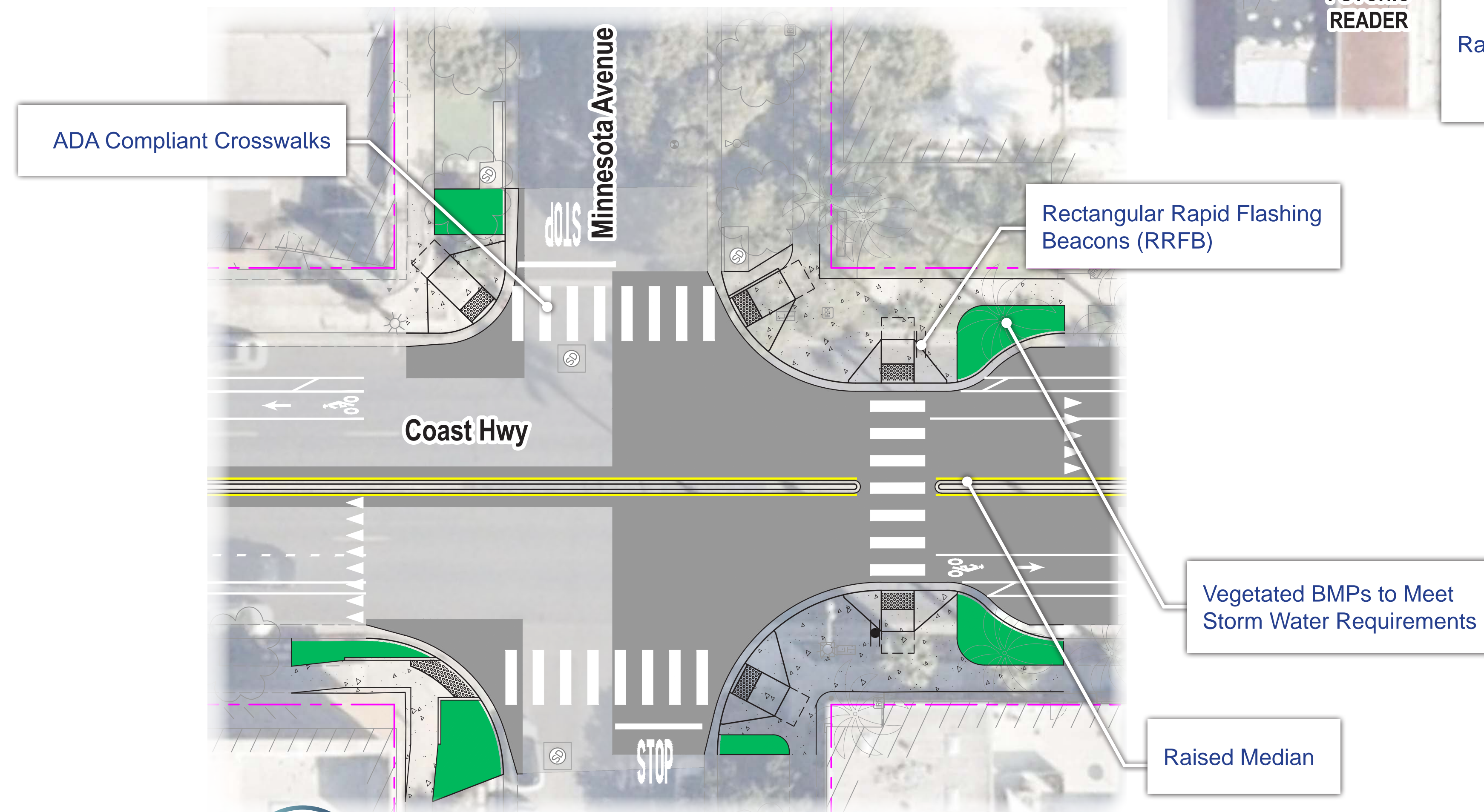
G MINNESOTA AVE - BULB-OUTS
