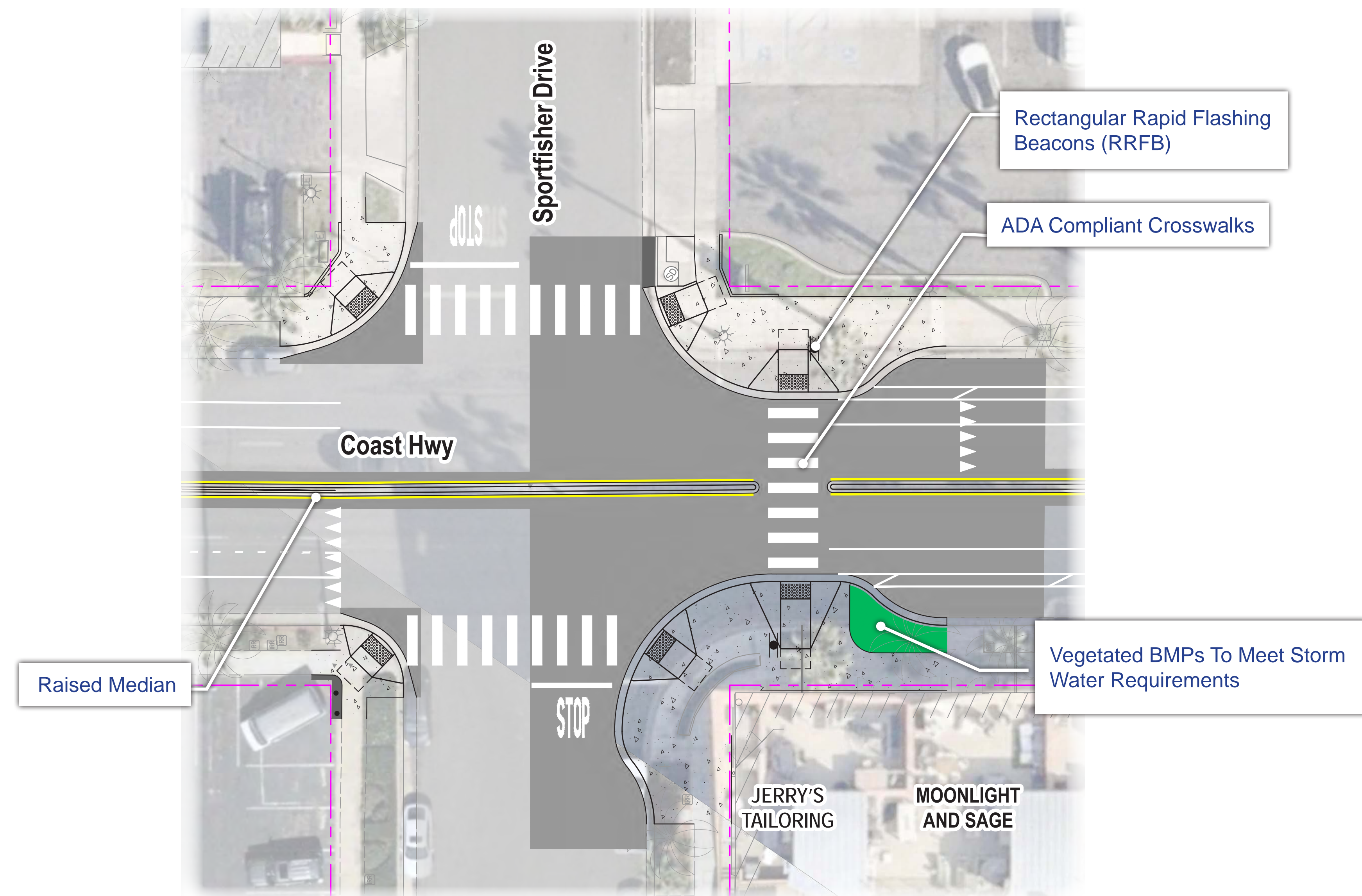
A SPORTFISHER DR - BULB-OUTS
