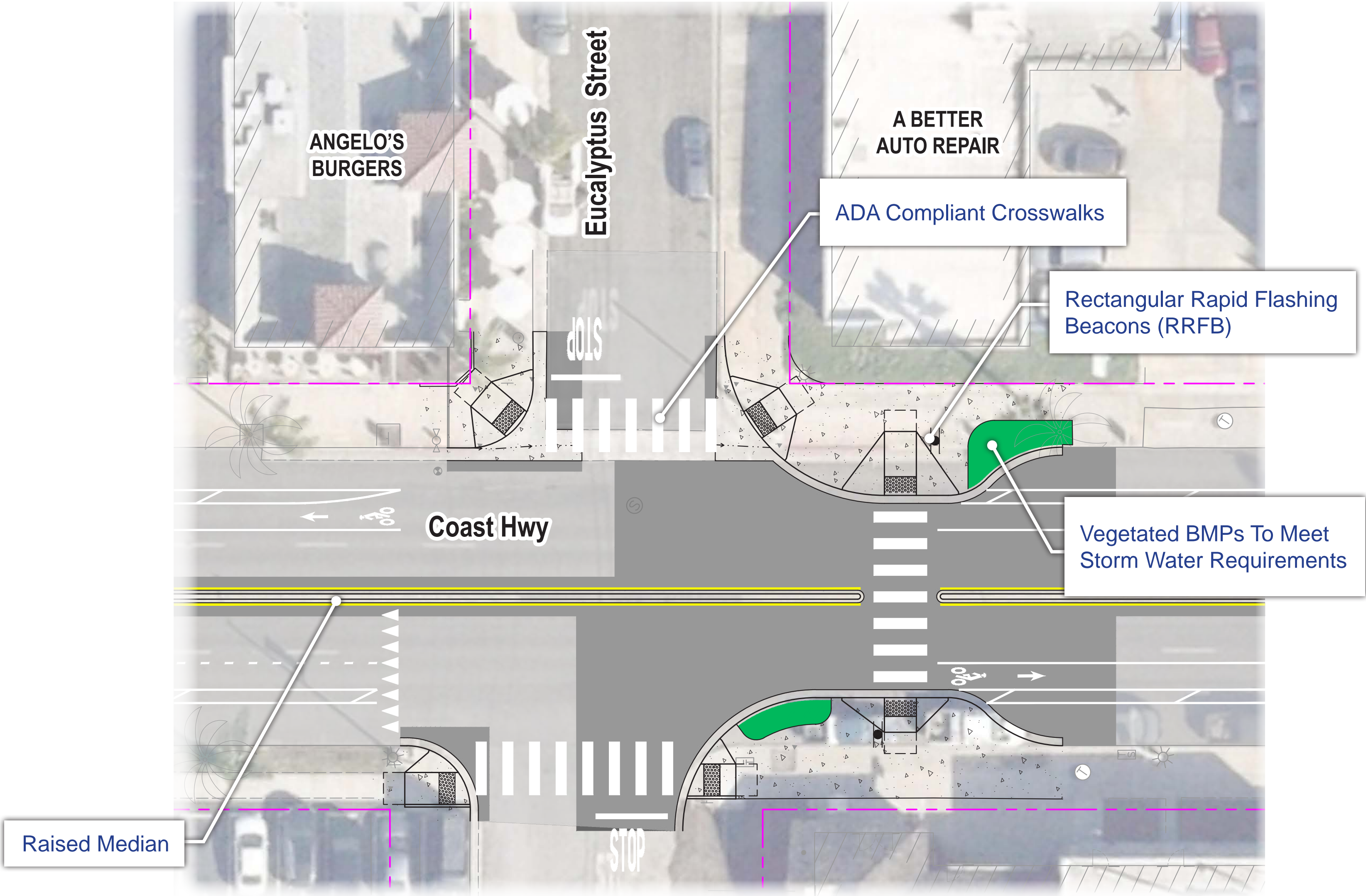
J EUCALYPTUS ST - BULB-OUTS
