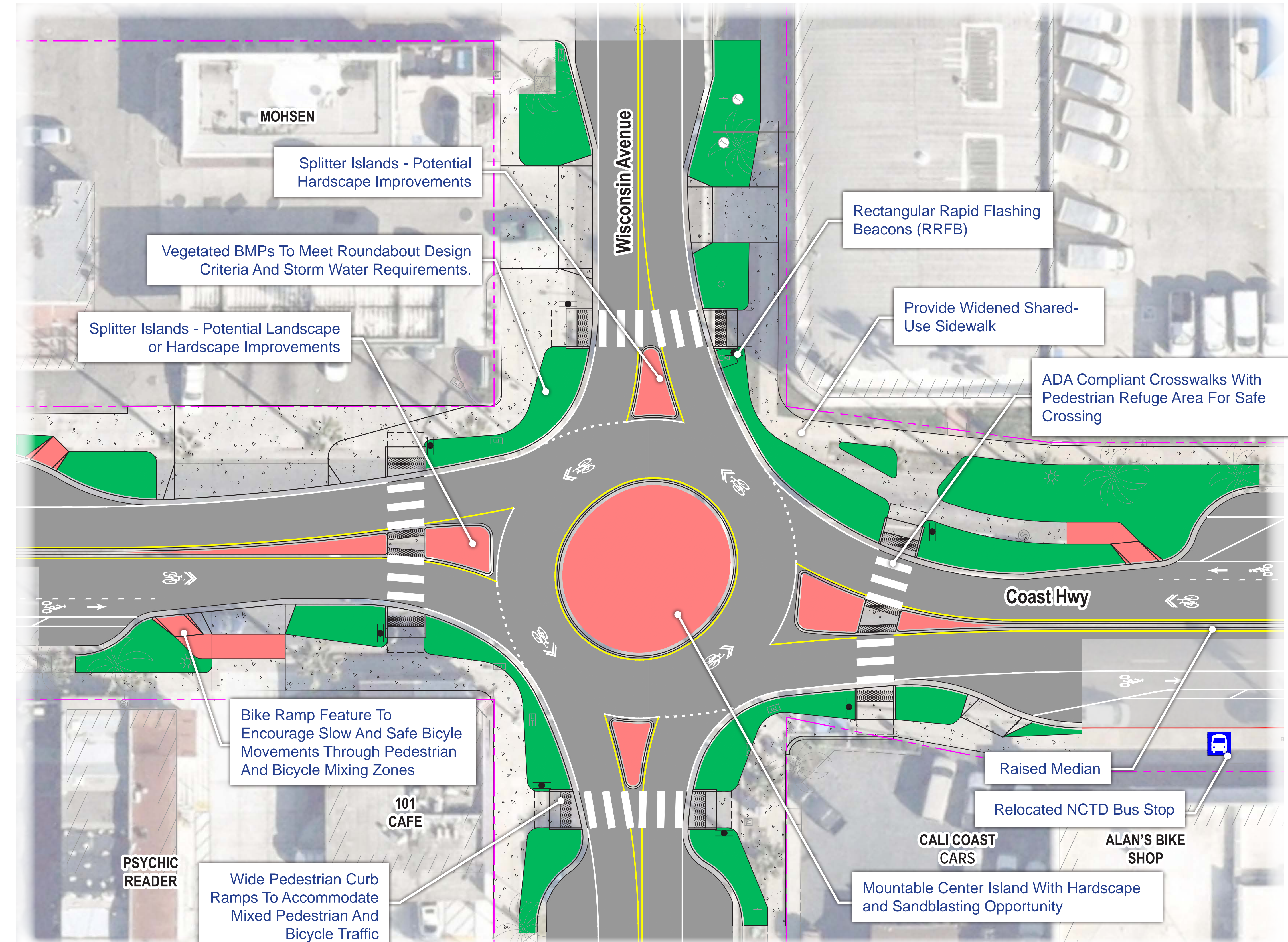
H WISCONSIN AVE - ROUNDABOUT
