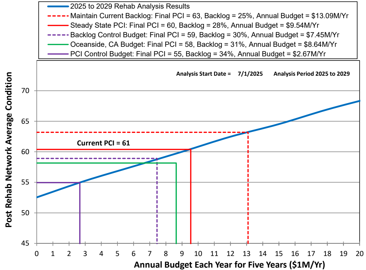
Figure 17 – Five-year Post Rehab Network PCI Analysis Results
