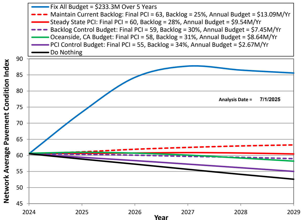
Figure 19 – Five-year Annual PCI
