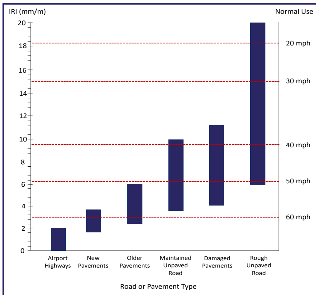
Figure 9 - IRI Scale Definitions
