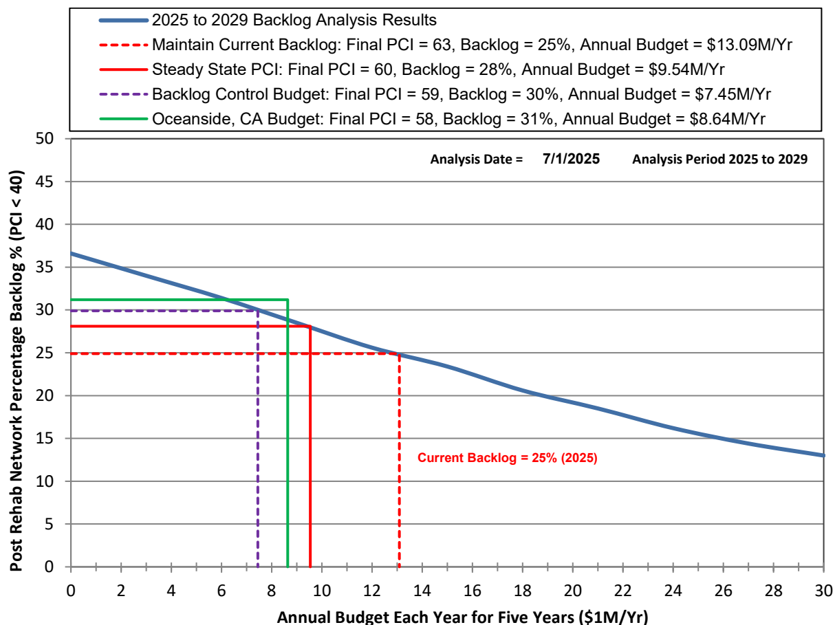
Figure 18 – Five-year Post Rehab Network Backlog Results
