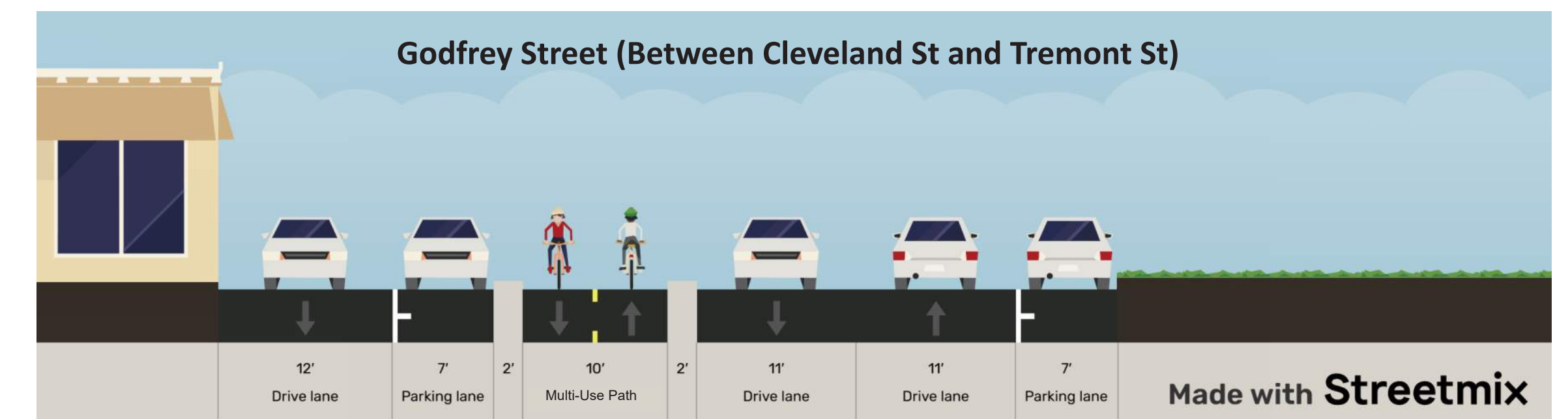
Cross-Section A-A: Proposed Conditions
