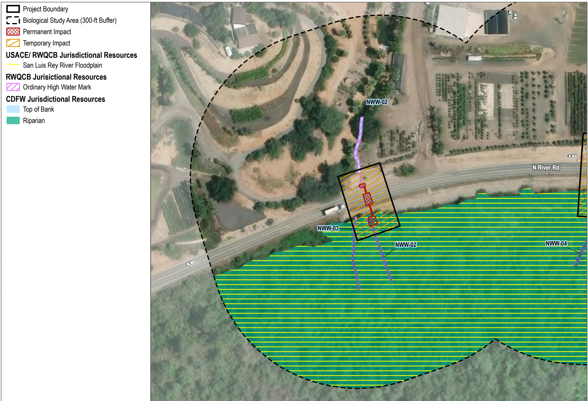
FIGURE 7c Impacts to Jurisdictional Resources - Culvert #3 North River Rd and Sleeping Indian Rd Drainage Improvements Project
