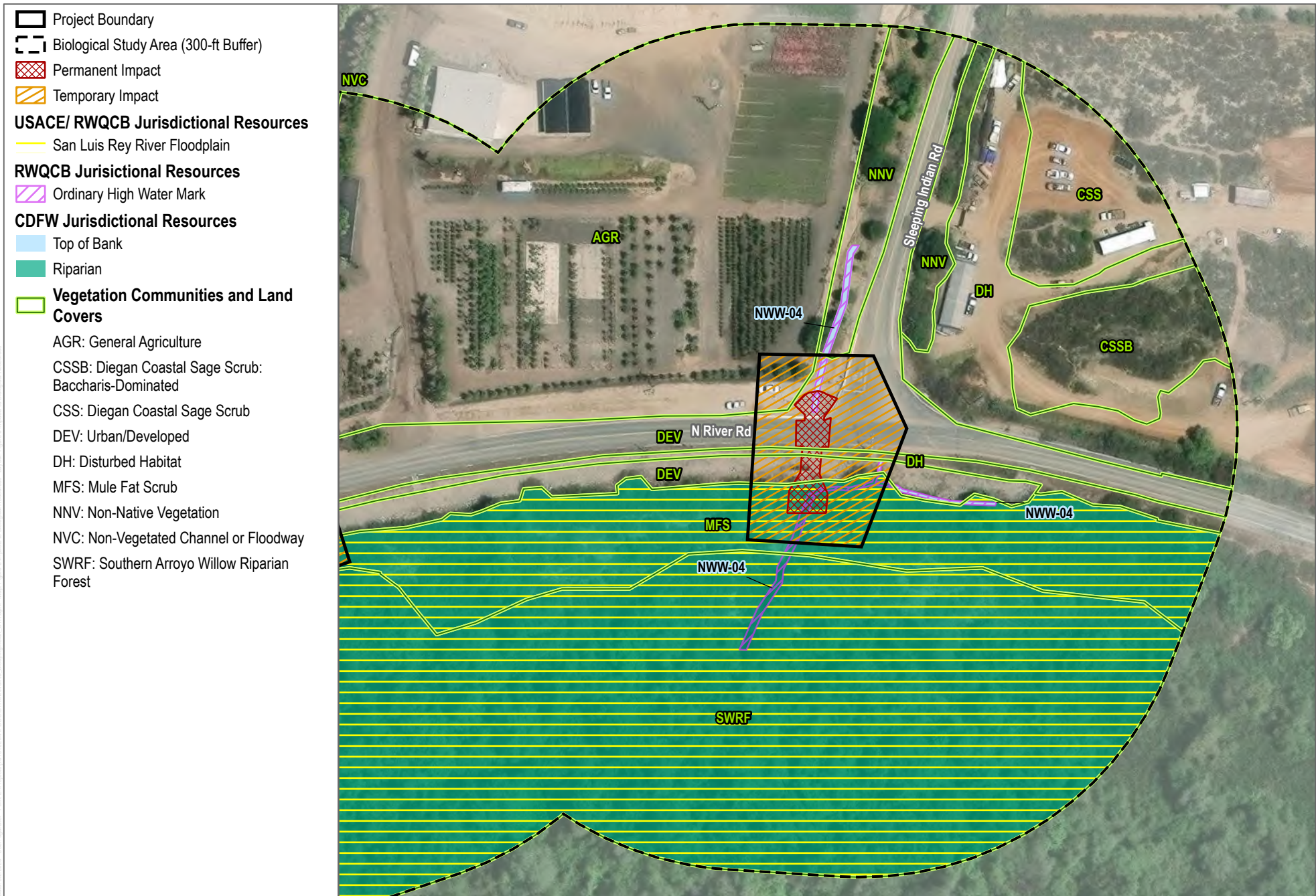
FIGURE 6b Impacts to Biological Resources - Culvert #2 North River Rd and Sleeping Indian Rd Drainage Improvements Project
